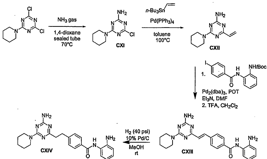
Scheme 32
